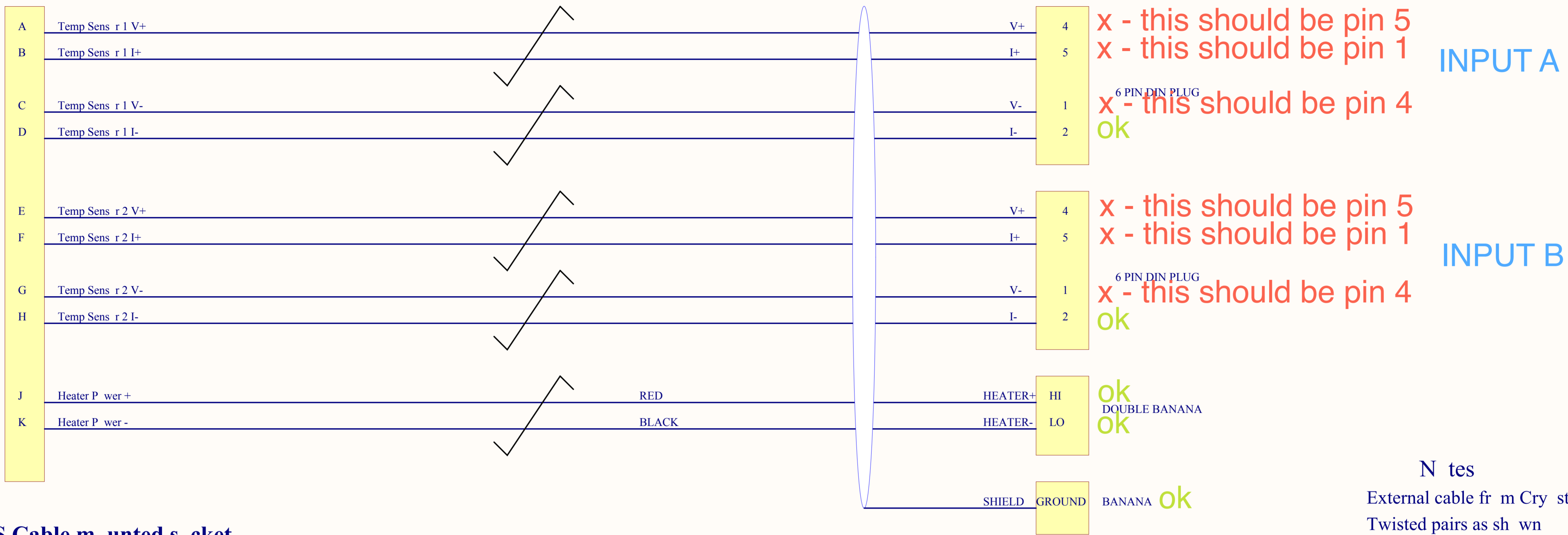
14-15S Cable mounted socket
